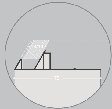
Top profile
